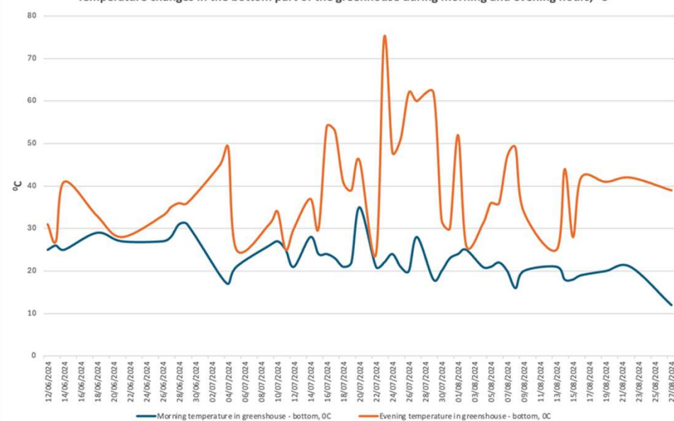
Temperature changes in the bottom part of the greenhouse during morning and evening hours, °C
